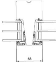
V4 Pfosten Fester Blendrahmen
